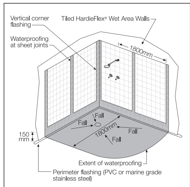
FIGURE 16 UNENCLOSED, TILED WALLS
