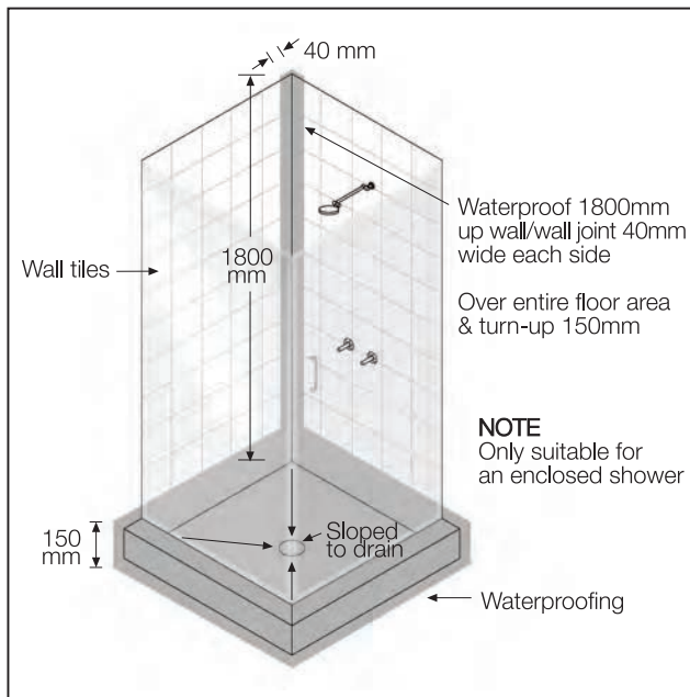
FIGURE 14 ENCLOSED SHOWER, TILED WALLS
