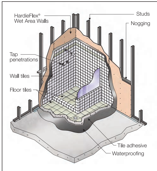
FIGURE 17 TYPICAL BATHROOM FINISH
