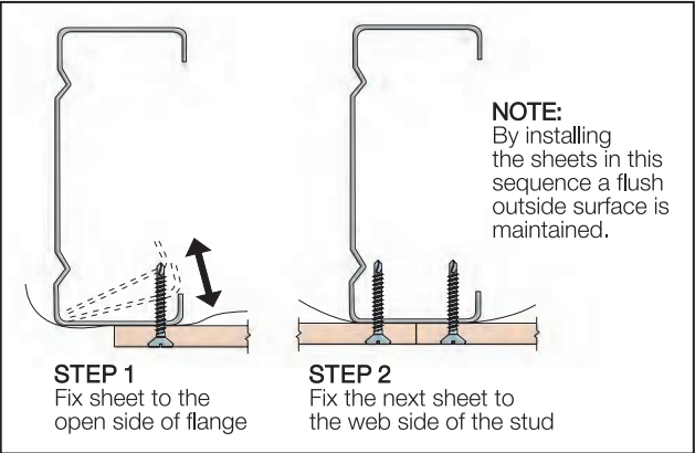
FIGURE 4 SCREW FASTENING
