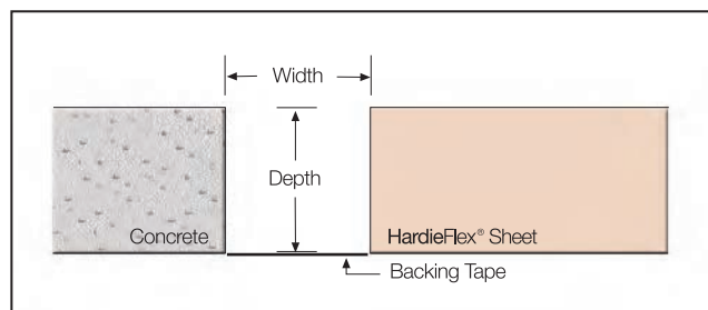
FIGURE 8 1:1 GAP
