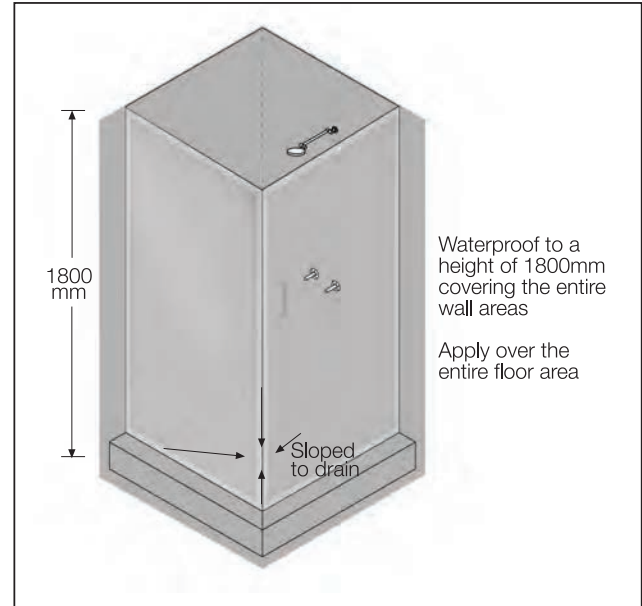
FIGURE 15 ENCLOSED SHOWER, TILED OR UNTILED WALLS
