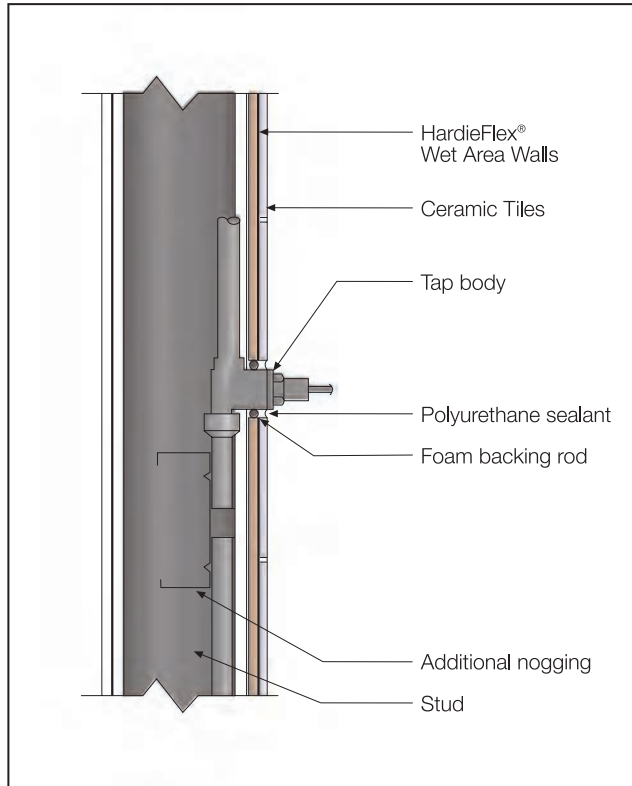
FIGURE 20 TYPICAL PLUMBING PENETRATION - SECTION
