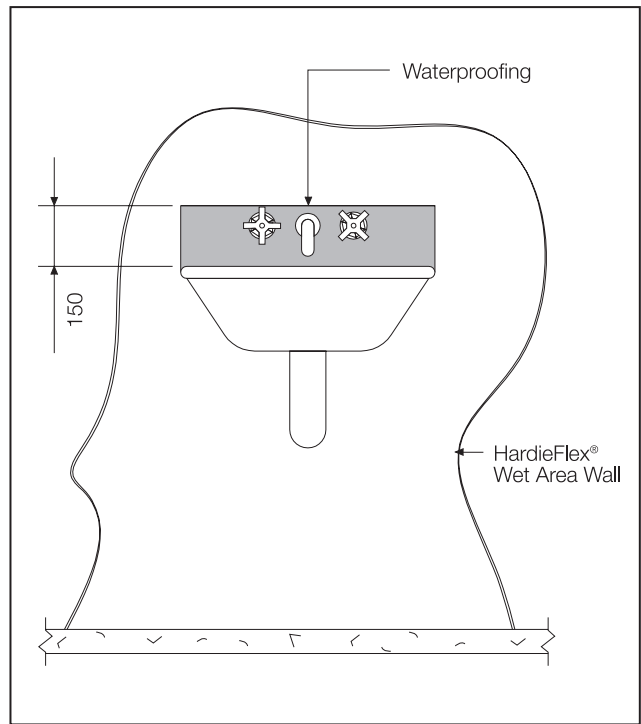
FIGURE 19 WATERPROOFING VESSELS ABUTTING WALLS
