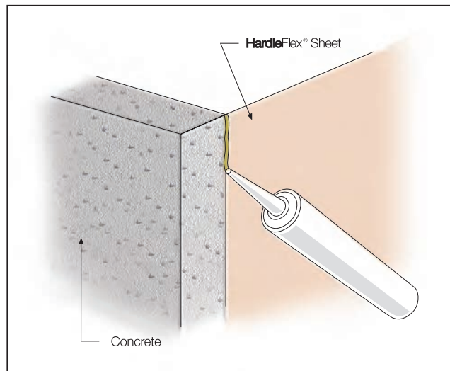
FIGURE 9 POLYURETHANE SEALANT
