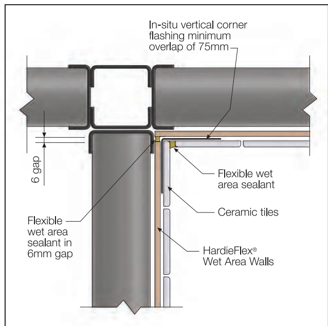
FIGURE 13 VERTICAL CORNER FLASHING
