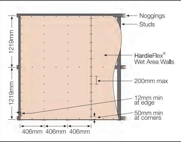
FIGURE 5 FASTENER SPACING
