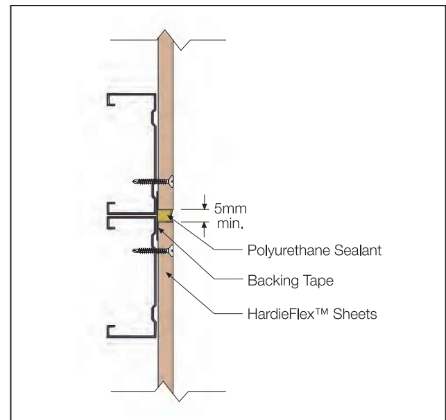
FIGURE 11 HORIZONTAL CONTROL JOINT
