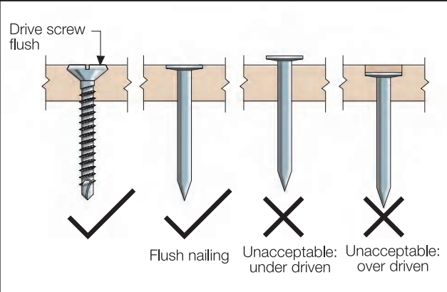
FIGURE 3 FASTENER DEPTH
