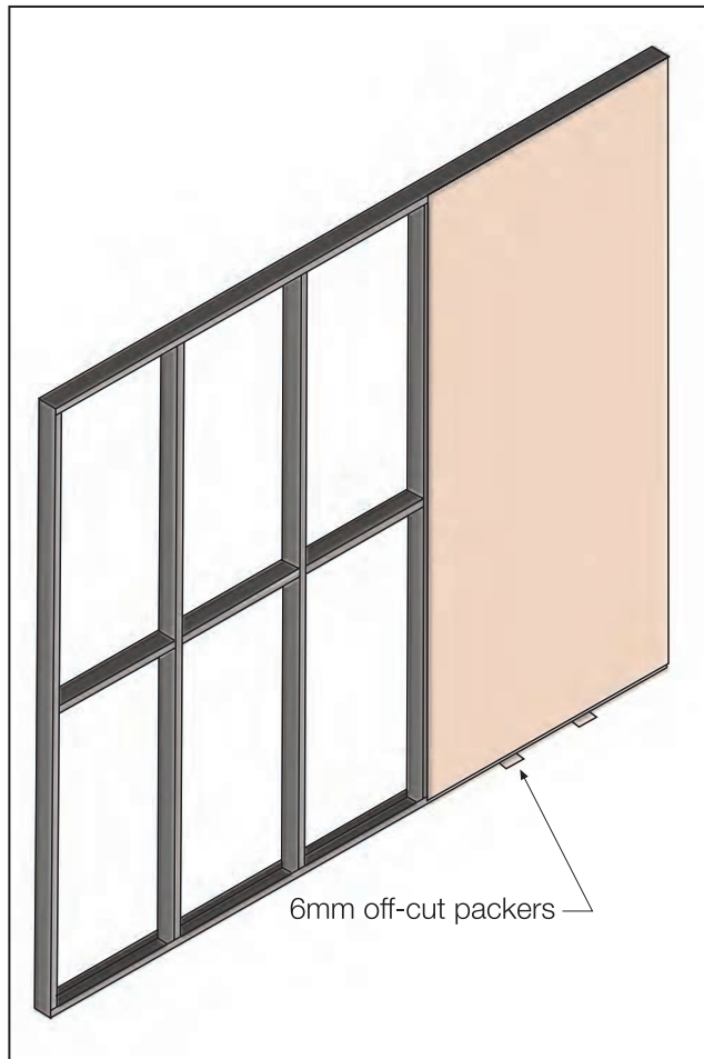
FIGURE 6 FIRST SHEET INSTALLATION
