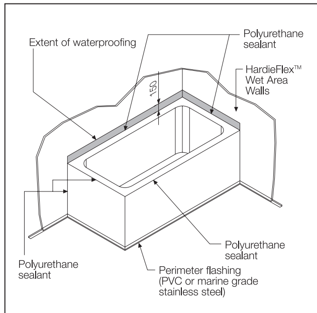
FIGURE 18 BATH WITHOUT SHOWER
