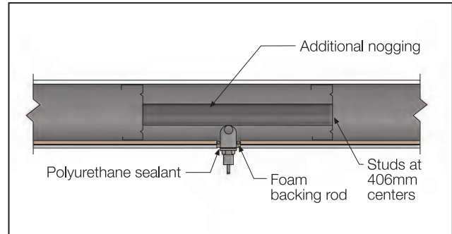
FIGURE 21 TYPICAL PLUMBING PENETRATION - PLAN
