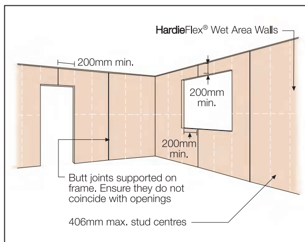
FIGURE 2 SHEET LAYOUT WITH DOOR AND WINDOW OPENING
