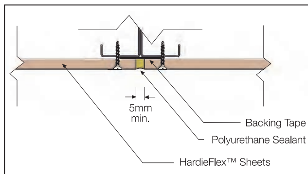
FIGURE 10 VERTICAL CONTROL JOINT
