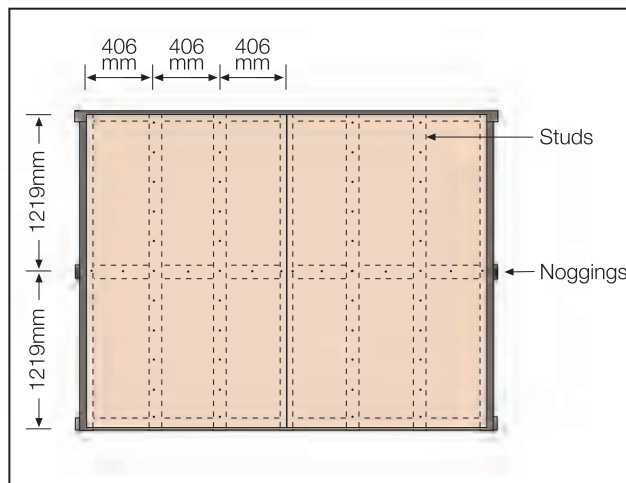
FIGURE 1 SHEET AND FRAME LAYOUT
