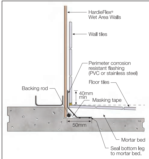
FIGURE 12 FLOOR/WALL JUNCTION FLASHING - OUTSIDE SHOWER AREA
